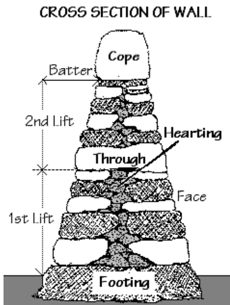
Fig.2. Typical wall cross section. After DSWA's “Techniques & Traditions” p.15.
