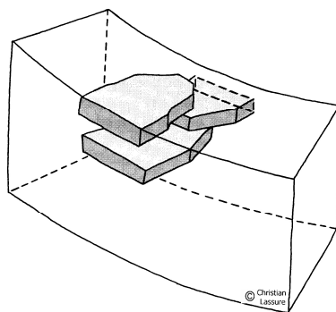
Fig.46. Illustration of horizontal key showing tail "held in a pincher grip by the tails of two headers" laid in opposite face. By kind permission. Christian Lassure "Building a drystone hut: an instruction manual". 2 nd Edition, C.E.R.A.V., 2009. p.15
