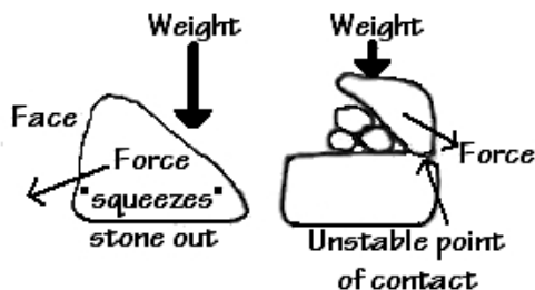
Fig.35. The problem of triangular profiles
