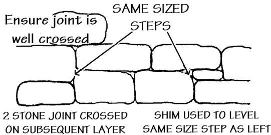
Fig.21. Shims versus double joints
