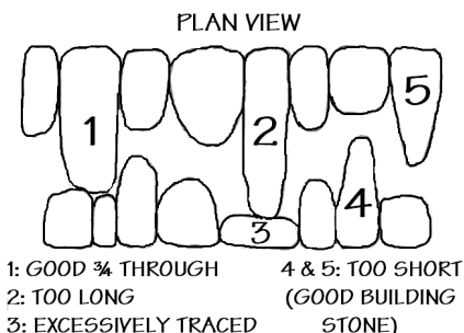
Fig.47. Appropriate and inappropriate use of stones as \frac{3}{4} throughs
